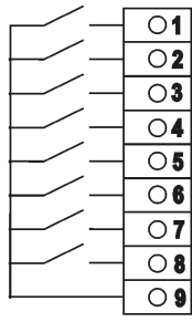
Relay Outputs
