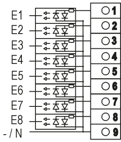
Signal Inputs
